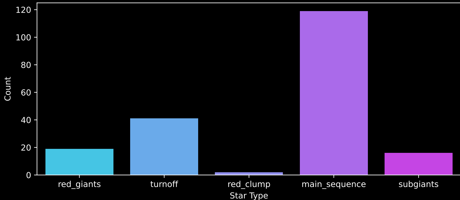
APOGEE DR17 Field: [110-62_MGA] Count plot of Star Type
