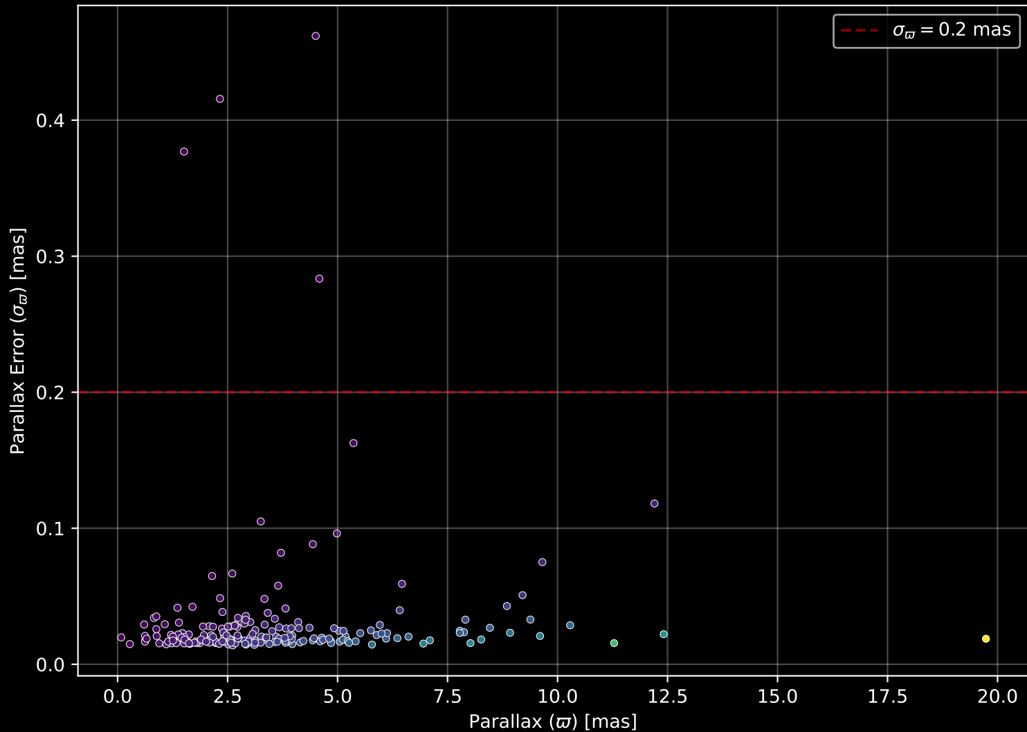
APOGEE DR17 Field: [110-62_MGA] Parallax Quality (n= 197)
