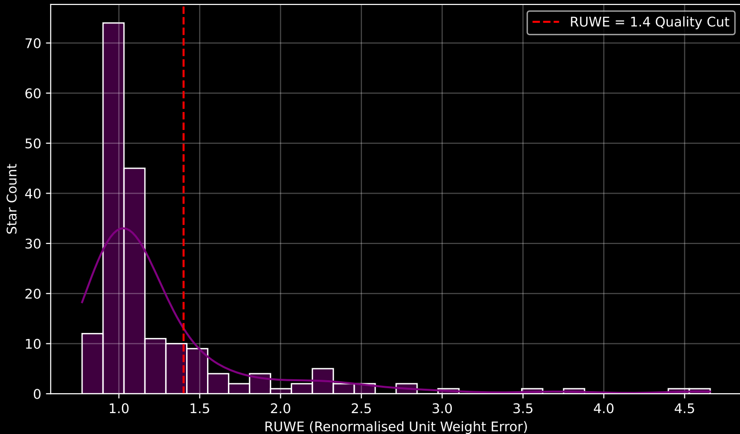
GAPOGEE DR17 Field [110-62_MGA] RUWE Distribution (n= 190)
