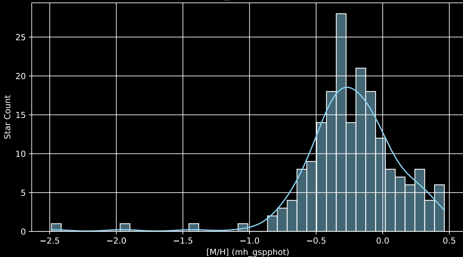
APOGEE DR17 Field: [110-62_MGA [M/H] (mh_gspphot) (n= 194)
