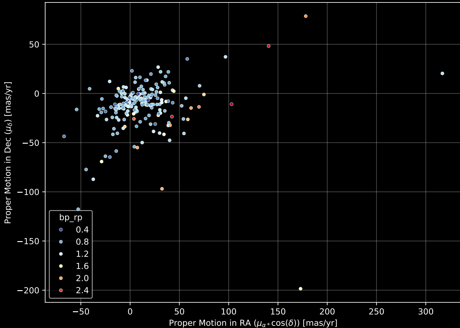
APOGEE DR17 Field: [110-62_MGA] Proper Motion Diagram (n= 197)
