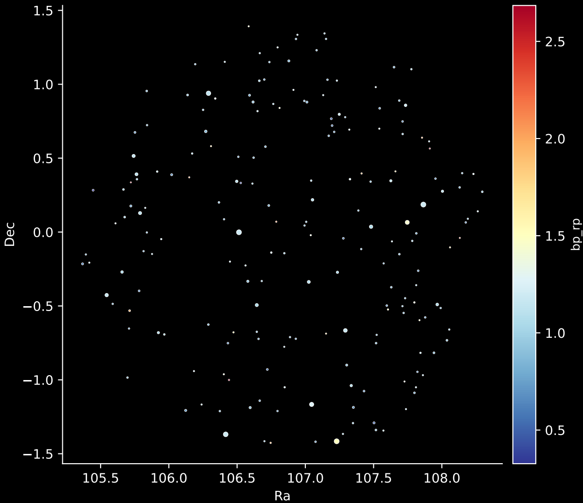
APOGEE DR17 Field: [110-62_MGA] Stars: 197
